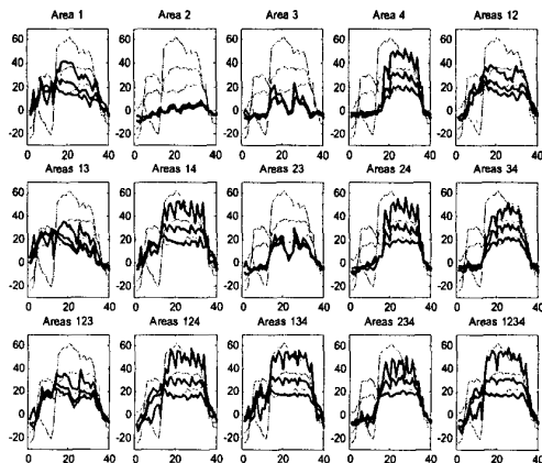
Figure 4. Wiener filter - Testing output X, Y, and Z trajectories (bold) for one desired movement (light) from fifteen Wiener filters trained with neuronal firing counts from all combinations of four cortical areas.
