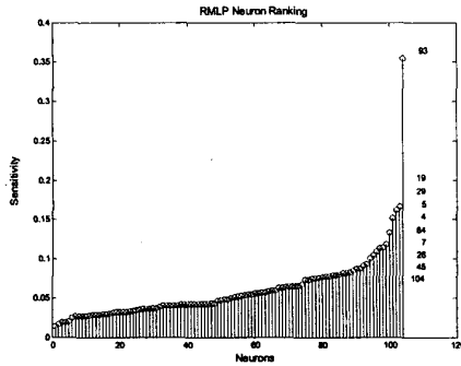
Figure 7. RMLP - Neuronal sensitivities sorted from minimum to maximum for a movement. The ten highest sensitivities are labeled with the corresponding neuron.
